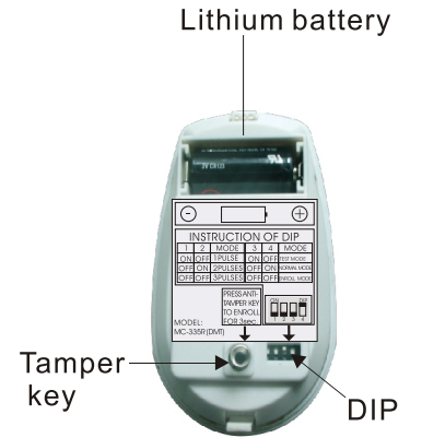
Fig. 2. Internal Structure
