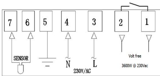
Voltage-Free System
